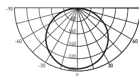
PBH-PC2-RS SENSOR 12w
